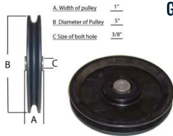
G. 5" PULLEY, 3/8" HOLE 5" Nylon Pulley for 1" frame with 3/8" bolt hole. Can be used with 1/4" or 3/16" cable. FW51B1H38
