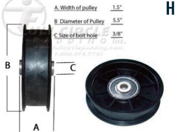
H. 5 1/2" PULLEY FOR BELTING 5 1/2" Pulley for 1-1/2" frame with a 3/8" bolt hole. Can be used with 15/16" belting. FW55FBB15H38
