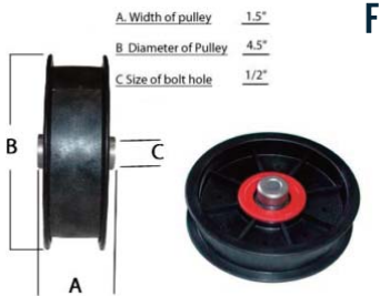
F. 4 1/2" PULLEY FOR BELTING 4 1/2" Pulley for 1-1/2" frame with a 1/2" bolt hole. Can be used with 15/16" belting FW45FBB15H12
