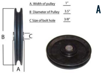
A. 3 1/2" PULLEY, 3/8" HOLE 3-1/2" pulley for 1" frame with 3/8" bolt hole. Can be used with 1/4" or 3/16" cable. FW35B1H38
