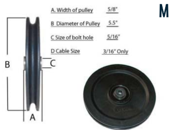
M. UNIVERSAL PULLEY - FOR OLDER UNIVERSAL EQUIPMENT ONLY Fits 3/16" Cable only UN720A
