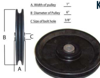
K. 6" PULLEY, 3/8" HOLE 6" Nylon Pulley for a 1" frame with 3/8" bolt hole. Can be used with either 1/4" or 3/16" cable. FW60B1H38
