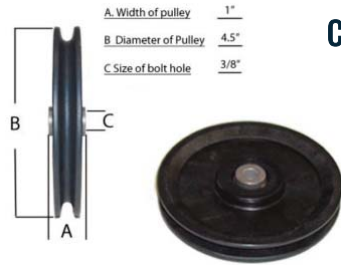
C. 4 1/2" PULLEY, 3/8" HOLE 4 1/2" pulley for 1" frame with 3/8" bolt hole. Can be used with 1/4" or 3/16" cable. FW45B1H38
