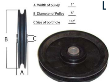
L. 6" PULLEY 1/2", HOLE 6" Nylon Pulley for a 1" frame with 1/2" bolt hole. Can be used with either 1/4" or 3/16" cable. FW60B1H12
