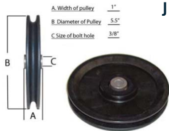
J. 5 1/2" PULLEY, 3/8" HOLE 5-1/2" Nylon pulley for a 1" frame with a 3/8" bolt hole. Can be used with 3/16" cable only. FW55B1H38
