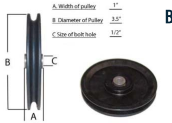
B. 3 1/2" PULLEY, 1/2" HOLE 3 1/2" pulley for 1" frame with 1/2" bolt hole. Can be used with 1/4" or 3/16" cable. FW35B1H12
