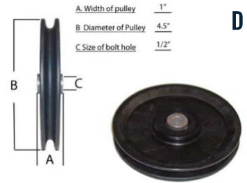
D. 4 1/2" PULLEY 1/2" HOLE 4 1/2" pulley for 1" frame with 1/2" bolt hole. Can be used with 1/4" or 3/16" cable. FW45B1H12
