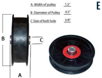
E. 4 1/2" PULLEY FOR BELTING 4-1/2" Pulley for 1 1/2" frame with a 3/8" bolt hole. Can be used with 15/16" belting. FW45FBB15H38
